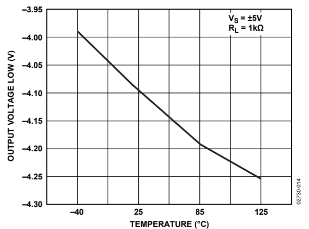
Figure 14. Output Voltage Low vs. Temperature at ±5 V
